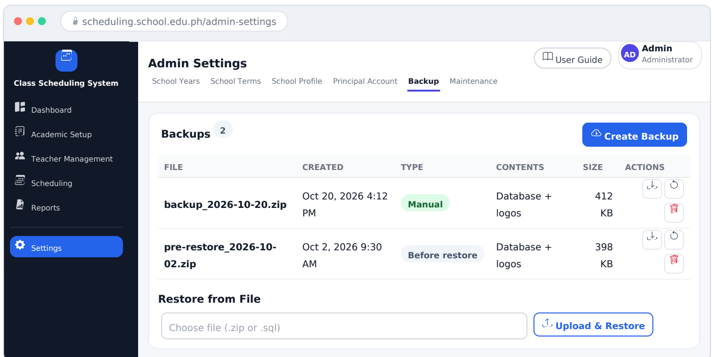
Figure 11. Backup tab.
